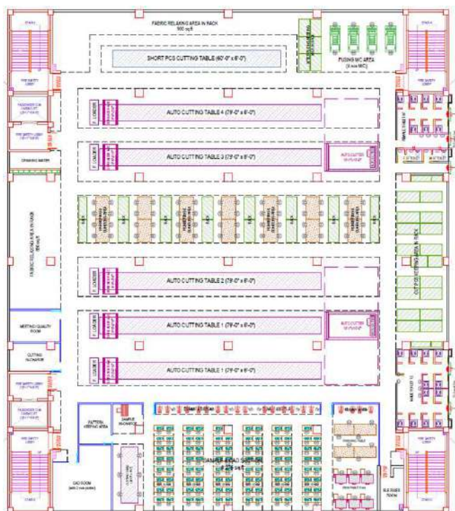
7 th FLOOR PLAN
