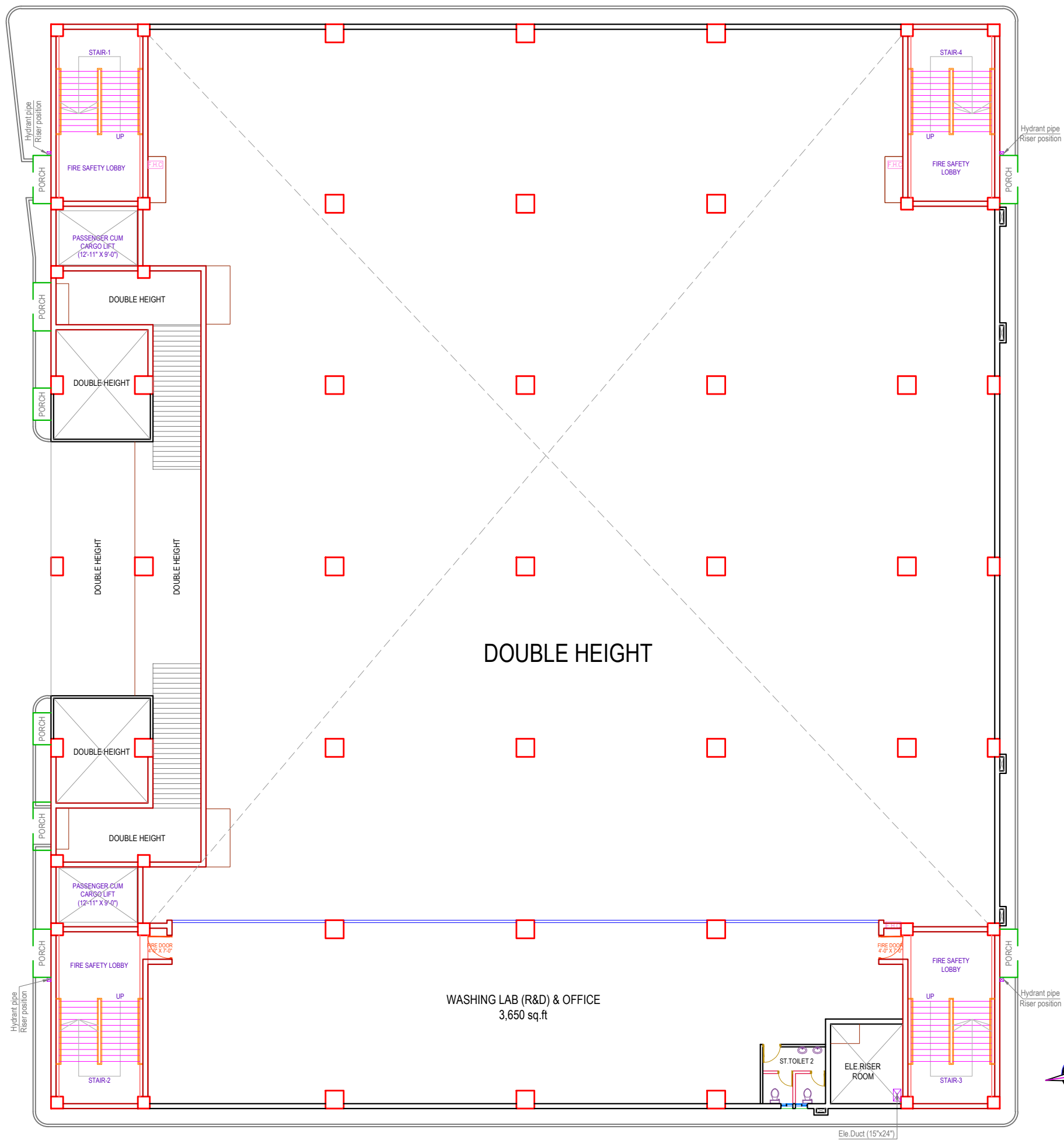
MEZZANINE FLOOR PLAN Floor area : 3,872 sq.ft
